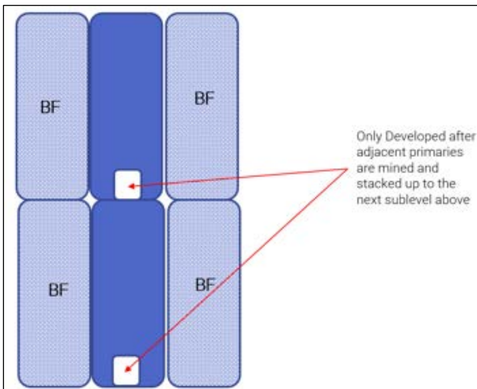
Figure 16-25: 1-3-5 Sublevel Vertical Sequence Section View
