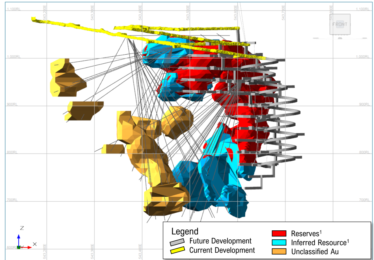
Horseshoe Underground Reserves, Resources and Growth Targets
